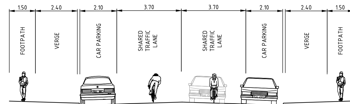
TYPICAL MID-BLOCK SECTION NOT TO SCALE
