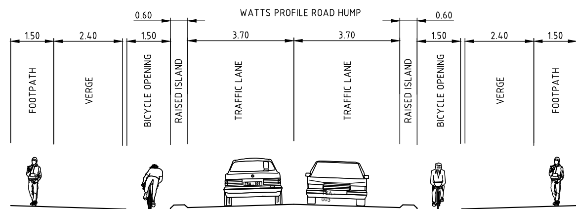
TYPICAL SECTION AT ROAD HUMP NOT TO SCALE
